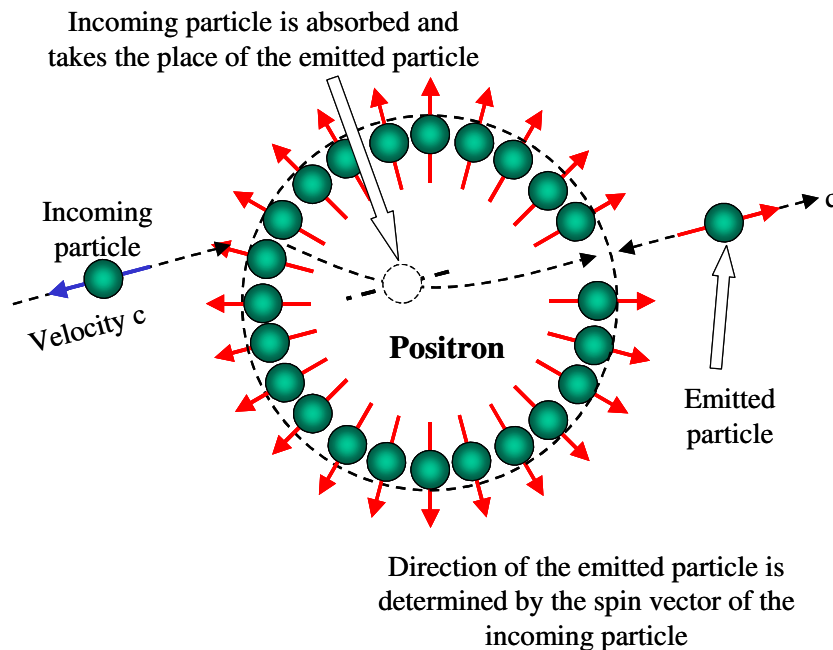
Figure 4. Showing interaction between a S^- particle and a positron
