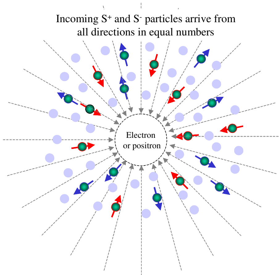
Figure 3. Neutral background showing Sp's arriving at an electron or positron
