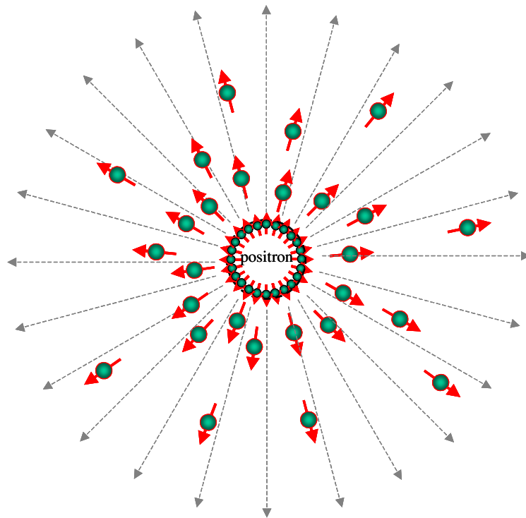
Figure 6. Space particles emitted from a positron.
