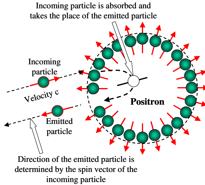
Figure 5. Showing interaction between a S^+ particle and a positron
