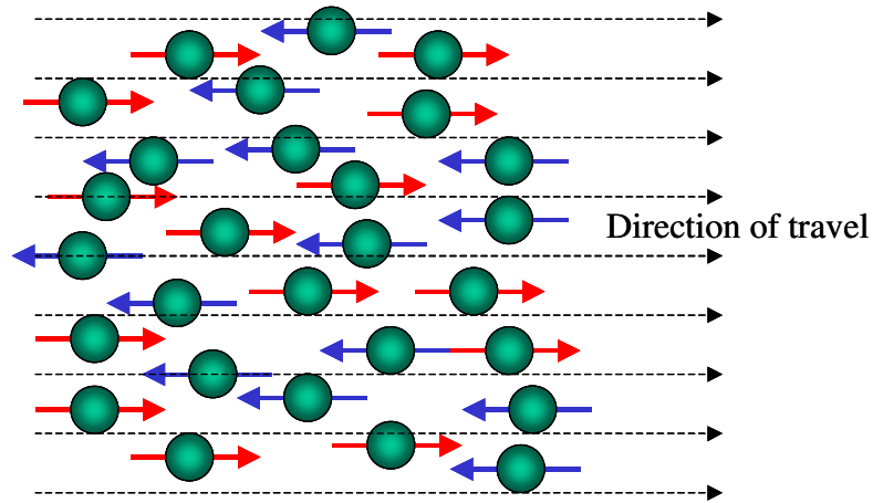
Figure 2. Neutral background of space particles.
