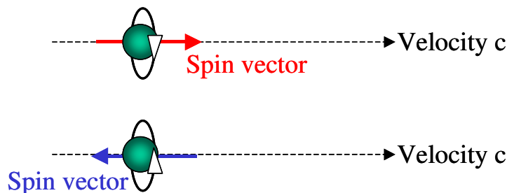
Figure 1. Space particles with positive and negative spin vectors
