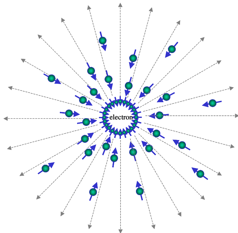
Figure 7. Space particles emitted from an electron.
