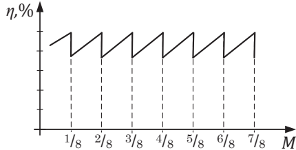
Fig. 4: Theoretical efficiency of the binary SCC.
