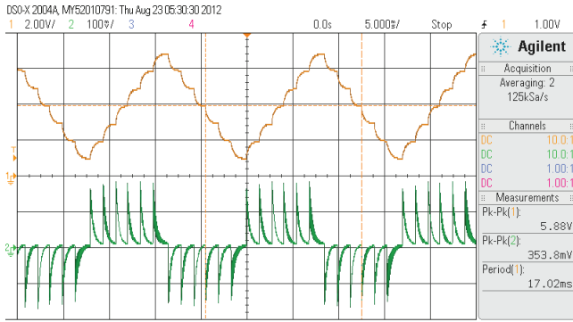
Fig 12: Experimental waveforms.
