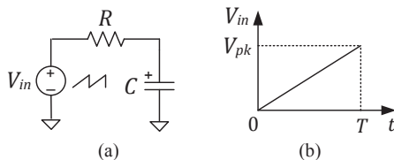
Fig 1: Circuit for linear charging (a) and the input voltage (b).
