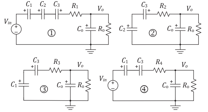
Fig. 5: Topologies of the binary SCC with the conversion ratio M_3=3/8 .
