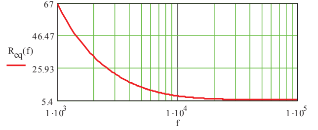
Fig. 9: R_{eq} as a function of f for the experimental SCC with M_3 = 3/8 .
