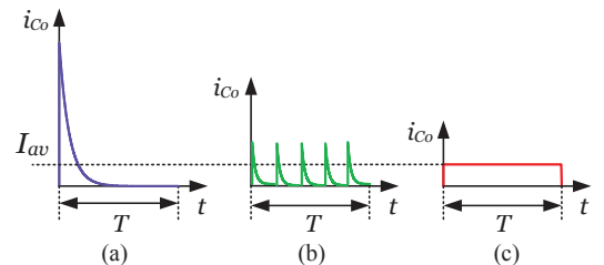
Fig. 7: Possible forms of momentary current through C_o .
