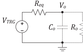
Fig. 3: The equivalent circuit of SCC.
