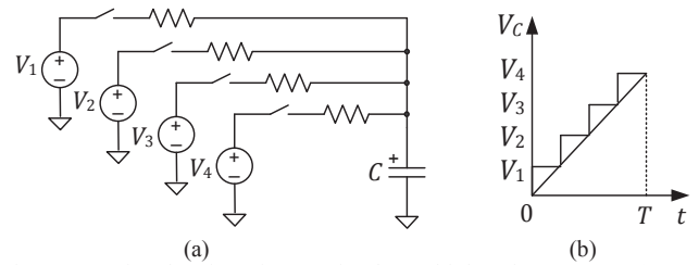
Fig. 2: Stepwise charging of a capacitor by multiple voltage sources (a) and the resulting stepped voltage (b).
