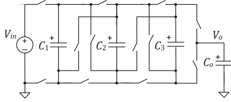
Fig 11: Switch network used in the binary SCC.
