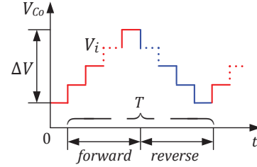
Fig. 6: Voltage across C_o in the proposed approach.
