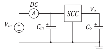
Fig. 10: Proposed experimental setup.
