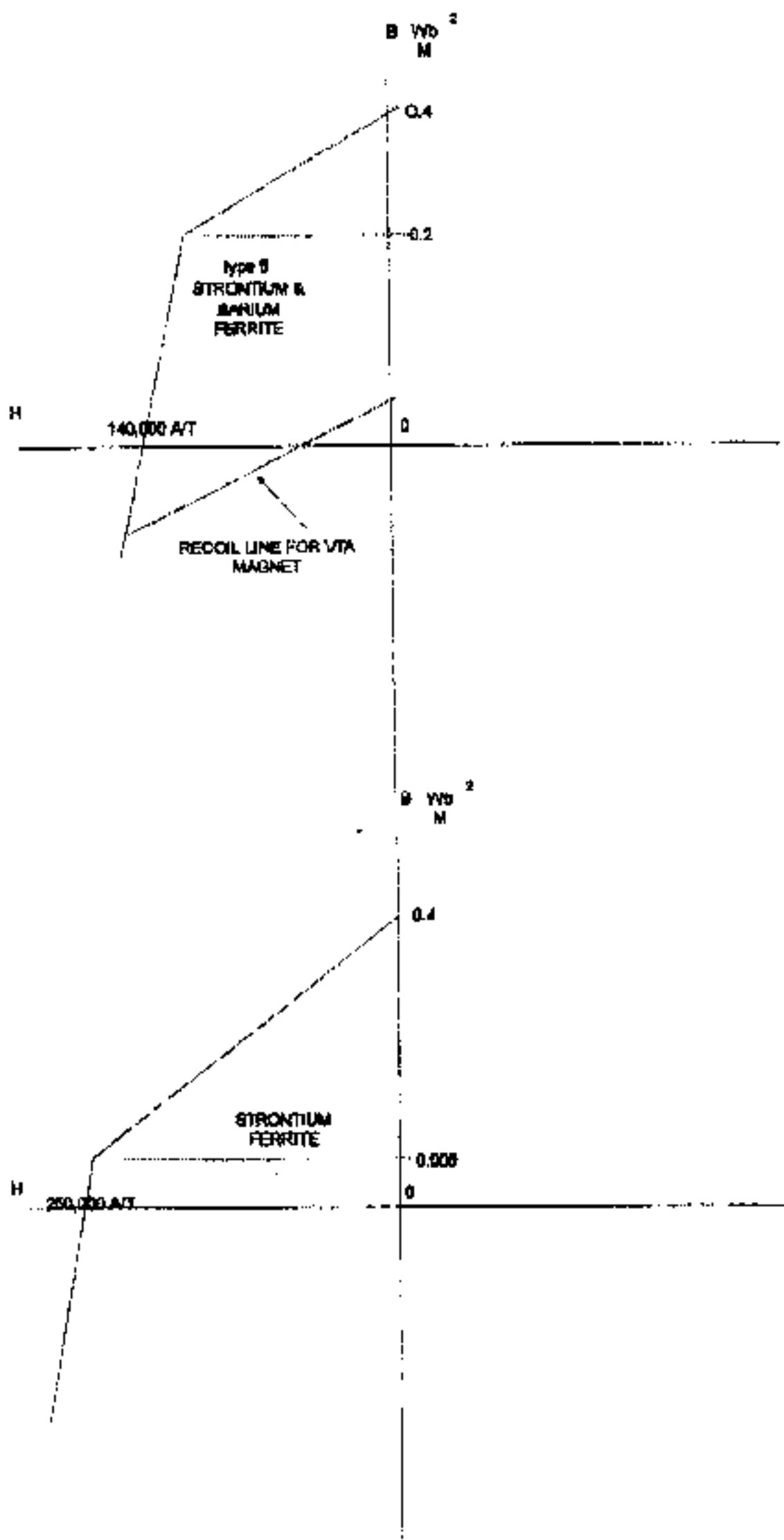
FIGURE 3 DEMAGNETISATION CURVES FOR STRONTIUM AND BARIUM FERRITE
