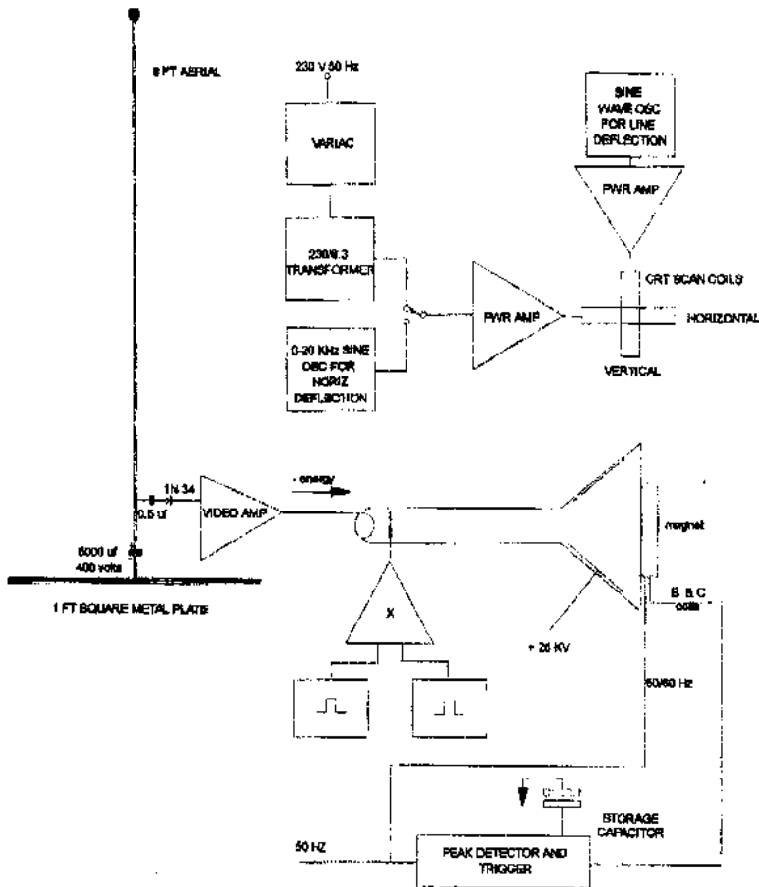
FIGURE 1 THE VTA CONDITIONING SYSTEM
