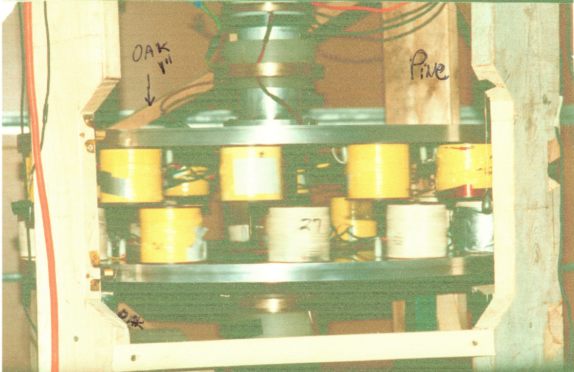
1.0" Thick oak stake cross brace.
