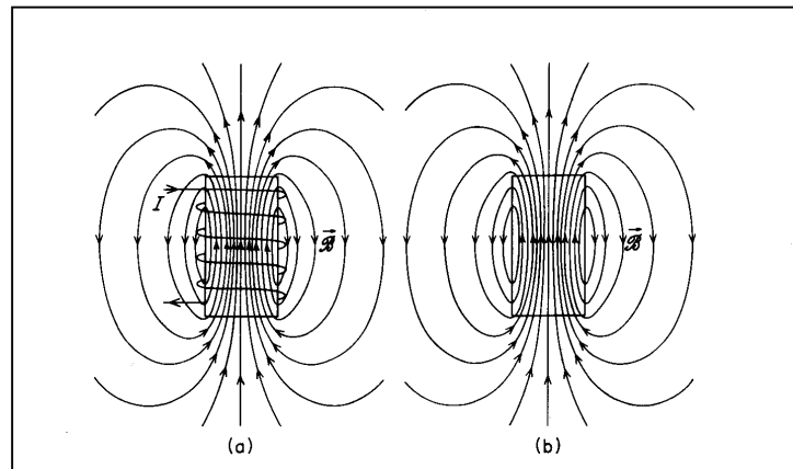
Figure 1. Magnetic field from (a) a solenoid and (b) a permanent magnet
