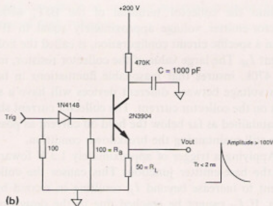
FIG. 1. (a) Typical I - V characteristics of planar epitaxial BJT. (b) Avalanche transistor pulse generator.
