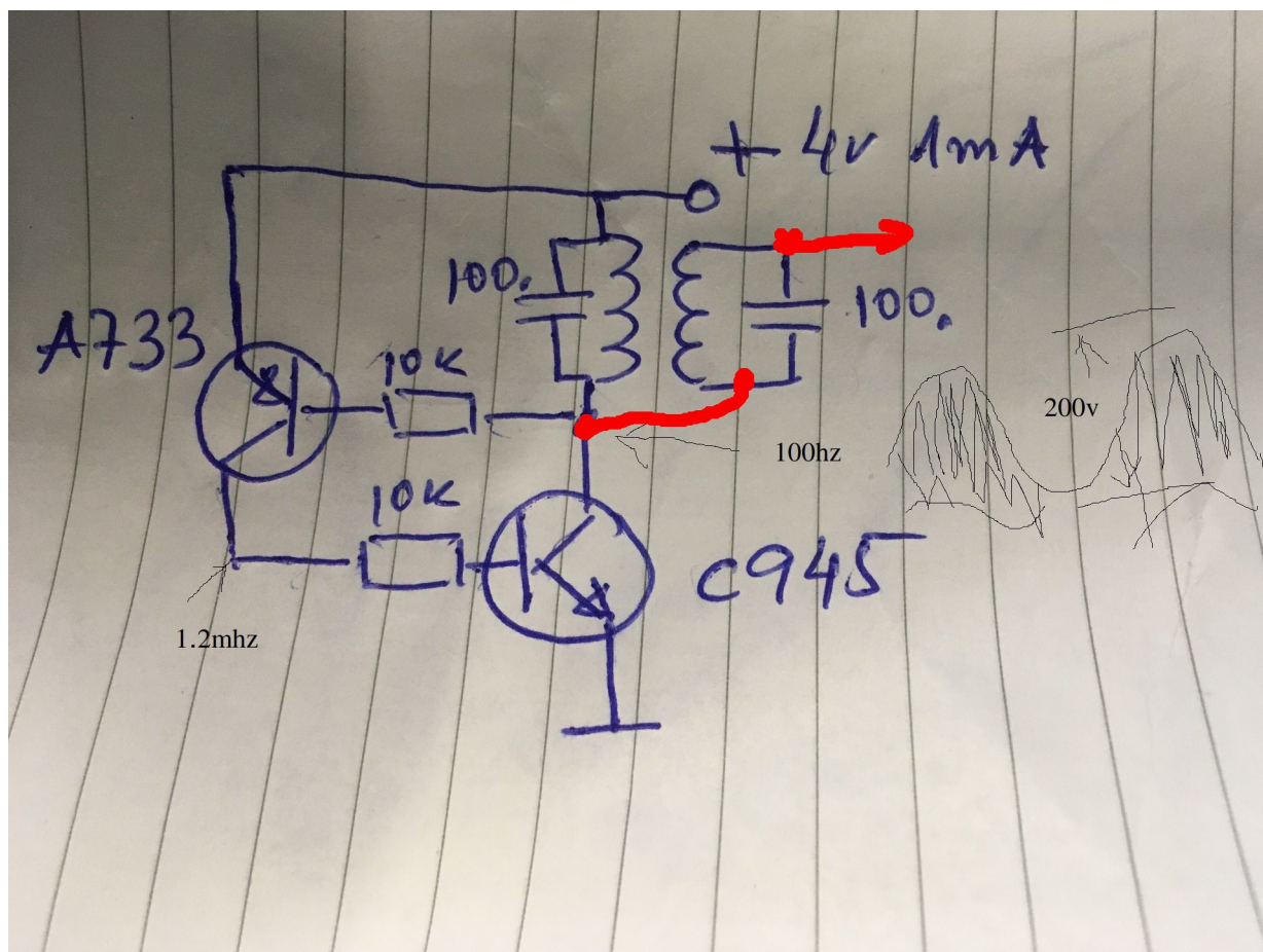
pic.4 same as 1,2,3 but with a regular transformer, pick up circuit not shown
