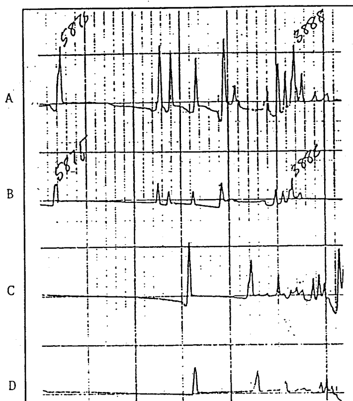
Spectrophotometer output for helium and water tube standards
