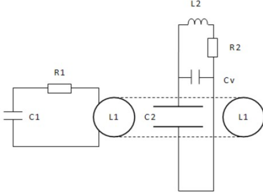
Fig. 2: Schematic of the two circuits. The circuit 1 is composed of C_1 , R_1 , and L_1 where L_1 is a toroidal solenoid. The circuit 2 is composed of C_2 , C_v , R_2 , and L_2 where C_2 is a parallel plate capacitor.
