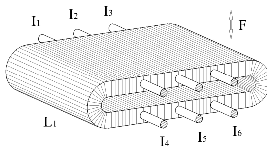
Figure 3. The three-dimensional schematic drawing of design optimization of Lorentz Force Propeller
