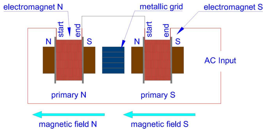
Figure 9: Testing the gathering of charges without secondary coil.
