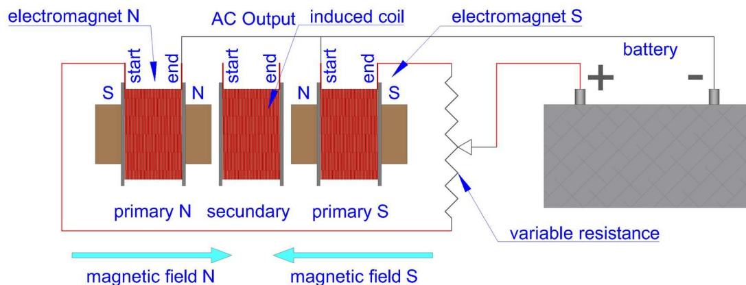
Figure 4: Simplified model of Figuera's device.
