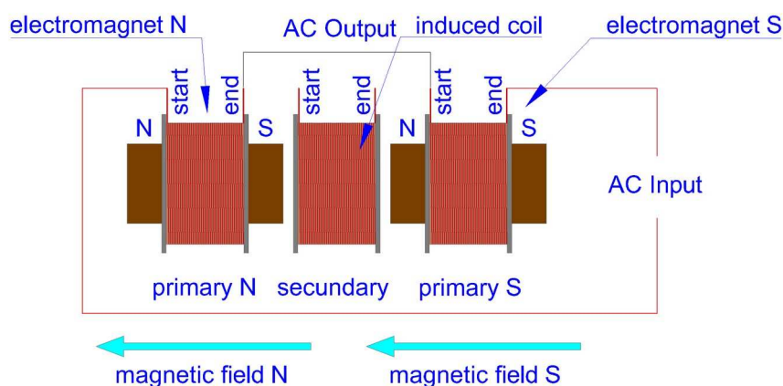
Figure 7: Testing a Figuera's simple device with AC.
