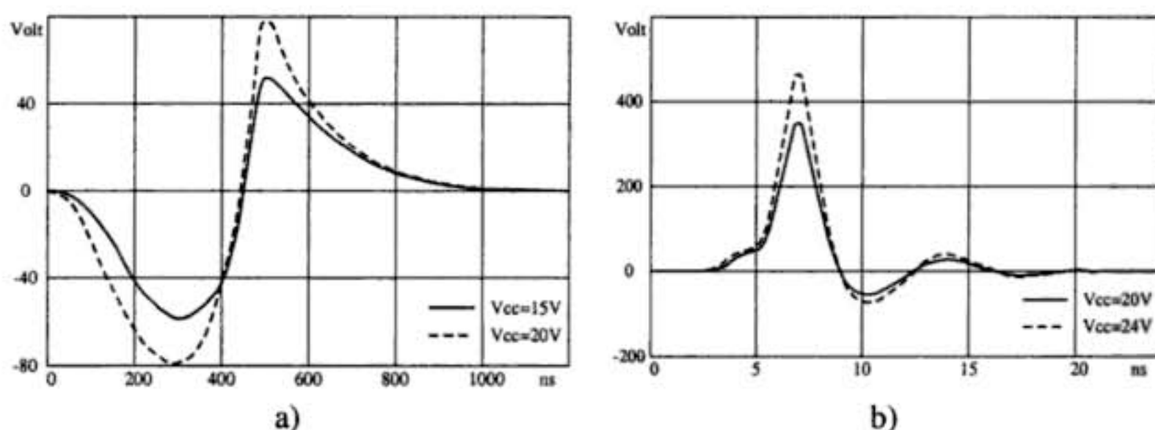
Figure 4. Output voltage waveform of the nanosecond pulse generator without DSRD (a) and when DSRD was connected to the loading (b).
