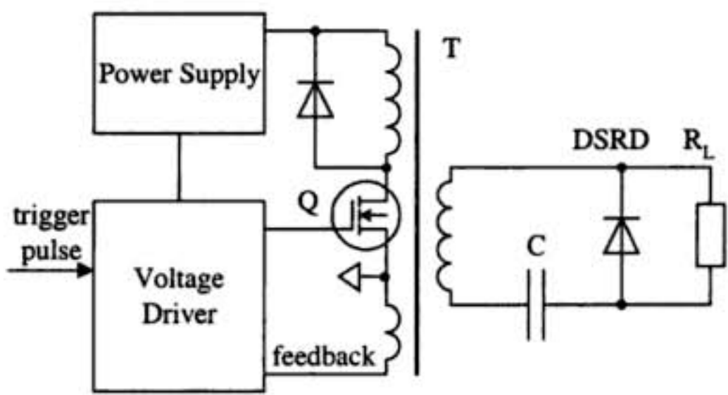
Figure 2. Simplified schematic diagram of the subnanosecond pulse generator based on DSRD sharpener.
